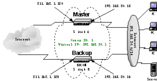
Figure1 0-1 Network topology
